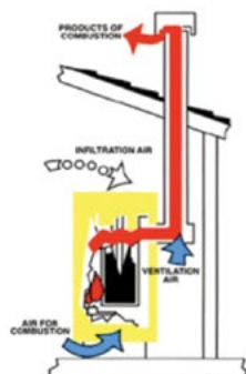
Conventional Vent
